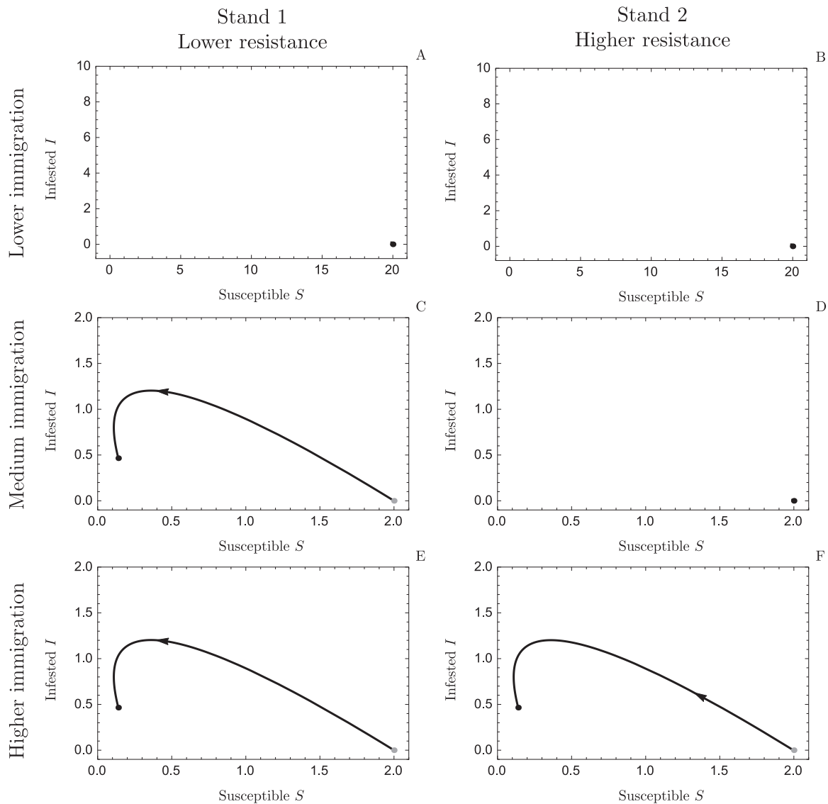
Fig. 3. The springboard effect of stand 1 on the beetle outbreak in stand 2. These plots assume that beetles disperse between two forest stands and there is an allochthonous beetle inflow to stand 1 (but not to stand 2). Stand 1 has a lower resistance ( r_1 = 30 ) when compared to stand 2 ( r_2 = 200 ). When immigration of beetles to stand 1 from outside of the system is relatively small (panels A, B; \mu_1 = 100 , \mu_2 = 0 ), both stands stay at the beetle-free state. For intermediate immigration rates to stand 1 (panels C, D; \mu_1 = 1000 , \mu_2 = 0 ), stand 1 shifts to the endemic equilibrium (12) while stand 2 stays at the beetle-free state. For high immigration rates to stand 1 (panels E, F; \mu_1 = 4000 , \mu_2 = 0 ), both stands shift to the endemic equilibrium. Besides the above differences, both stands are assumed to be identical. The curve is a trajectory of model (16) when beetles distribute uniformly over available trees. The black dot denotes a locally stable equilibrium, while the gray dot denotes an unstable equilibrium. Untransformed parameters used for simulations: \beta_0 = 0.01 , \lambda_1 = \lambda_2 = 0.001 , g_1 = g_2 = 0.001 , r_1 = r_2 = 0.1 , m_1 = m_2 = 0.05 , d_1 = d_2 = 0.003 , K_1 = K_2 = 100 , \delta = 10 , e = 10 . For simulations these parameters were non-dimensionalized following scheme in Table 3.
