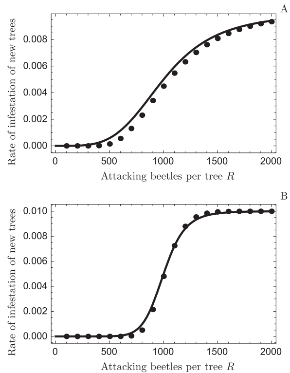
Fig. C1. Comparison of the rate of infestation of new trees (C.1) (dots) and its approximation by the Hill model (3) (line). Model (C.1) assumes a Negative Binomial distribution with \theta = 1000 and dispersion parameter k = 7 in panel A and k = 50 in panel B. Model (3) assumes r = 1000 and n = 4 in panel A and n = 10 in panel B. In both panels \beta_0 = 0.01 .
