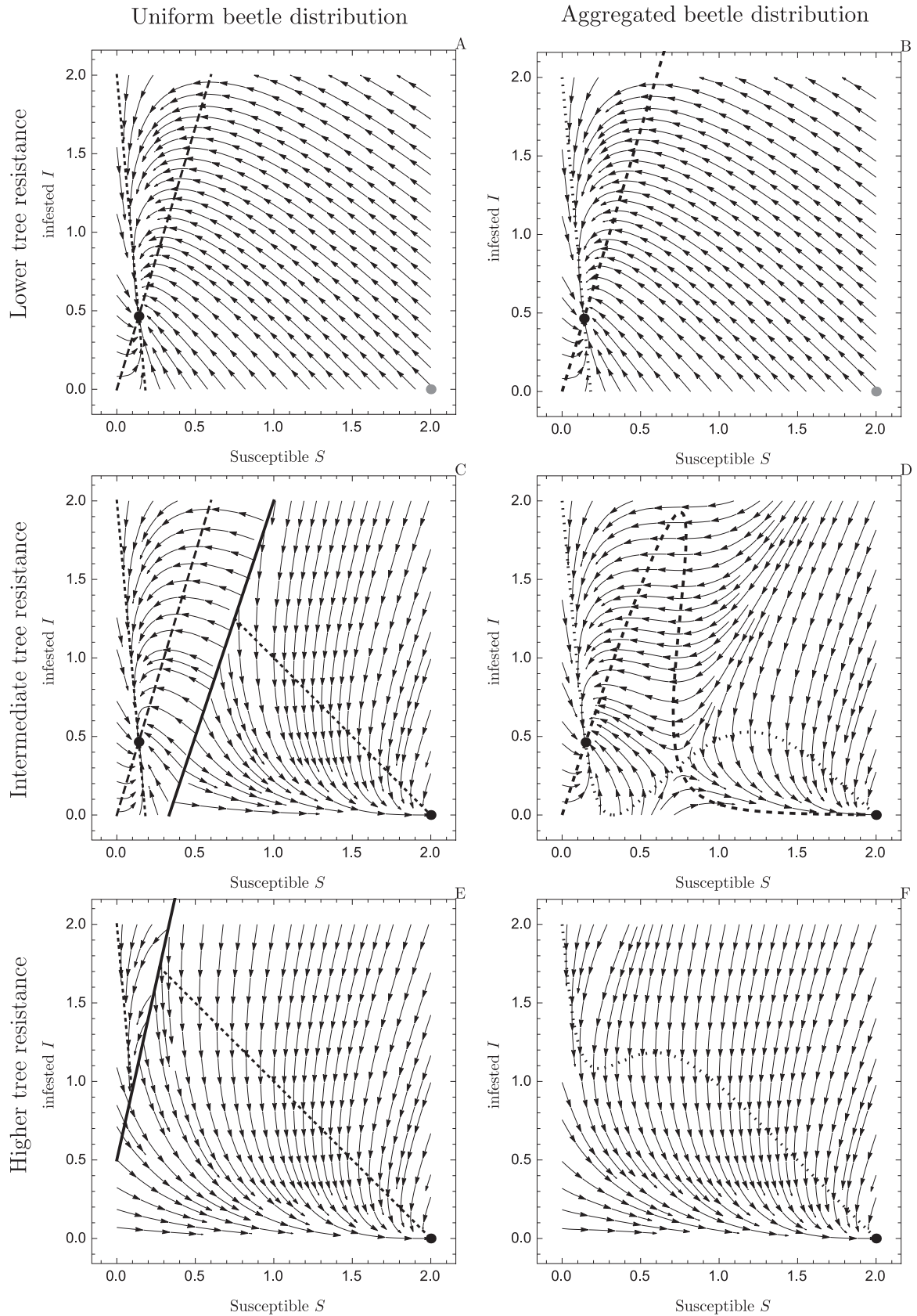
Fig. 1. These plots show trajectories of model (6) for uniform beetle distribution ( \beta is given by (8)) (left panels) and aggregated beetle distribution ( \beta is given by (7) with n=10 ) (right panels). Panels A and B assume low tree resistance ( r=30 ), panels C and D assume intermediate resistance ( r=300 ), and panels E and F assume high resistance ( r=450 ). The solid line in panels C and E is the threshold I_{min} for infestation given by (9) above which beetle spread in the forest. The dotted line is the isocline for susceptible trees and the dashed line is the isocline for infested trees. The black dot denotes a locally stable equilibrium, while the gray dot denotes an unstable equilibrium. Other untransformed parameters are g=0.001 , d=0.003 , m=0.05 , \beta_0=0.01 , \mu=2000 , K=100 . For simulations these parameters were non-dimensionalized following scheme in Table 3.
