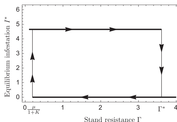
Fig. 2. Dependence of the equilibrium infestation I^* on the transformed stand resistance. This figure documents hysteresis in the forest dynamics. Untransformed parameters: g=0.001 , d=0.003 , m=0.05 , \beta_0 = 0.01 , \mu = 2000 , K=1000 . For simulations these parameters were non-dimensionalized following scheme in Table 3.
